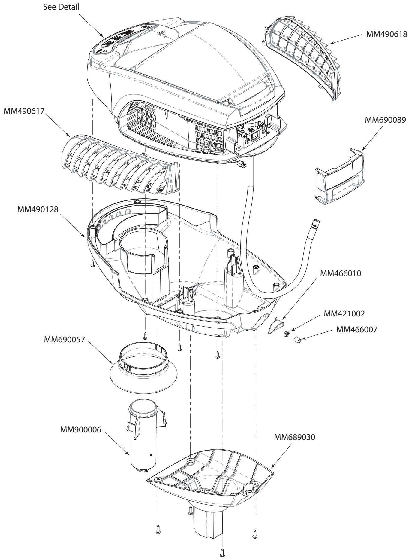
Power Pack Assy
