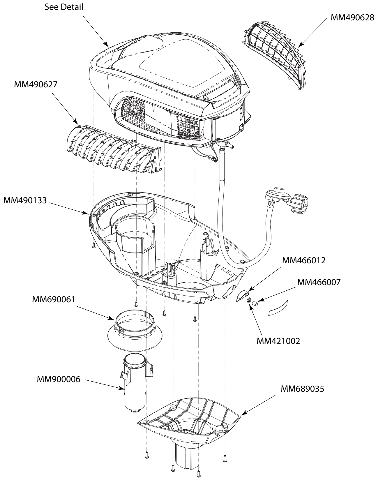
Power Pack Assy
