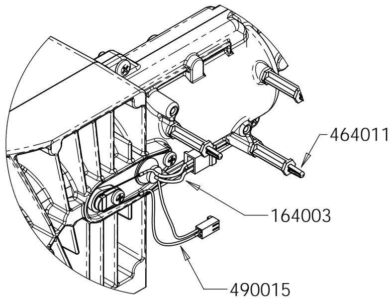
DETAIL A
