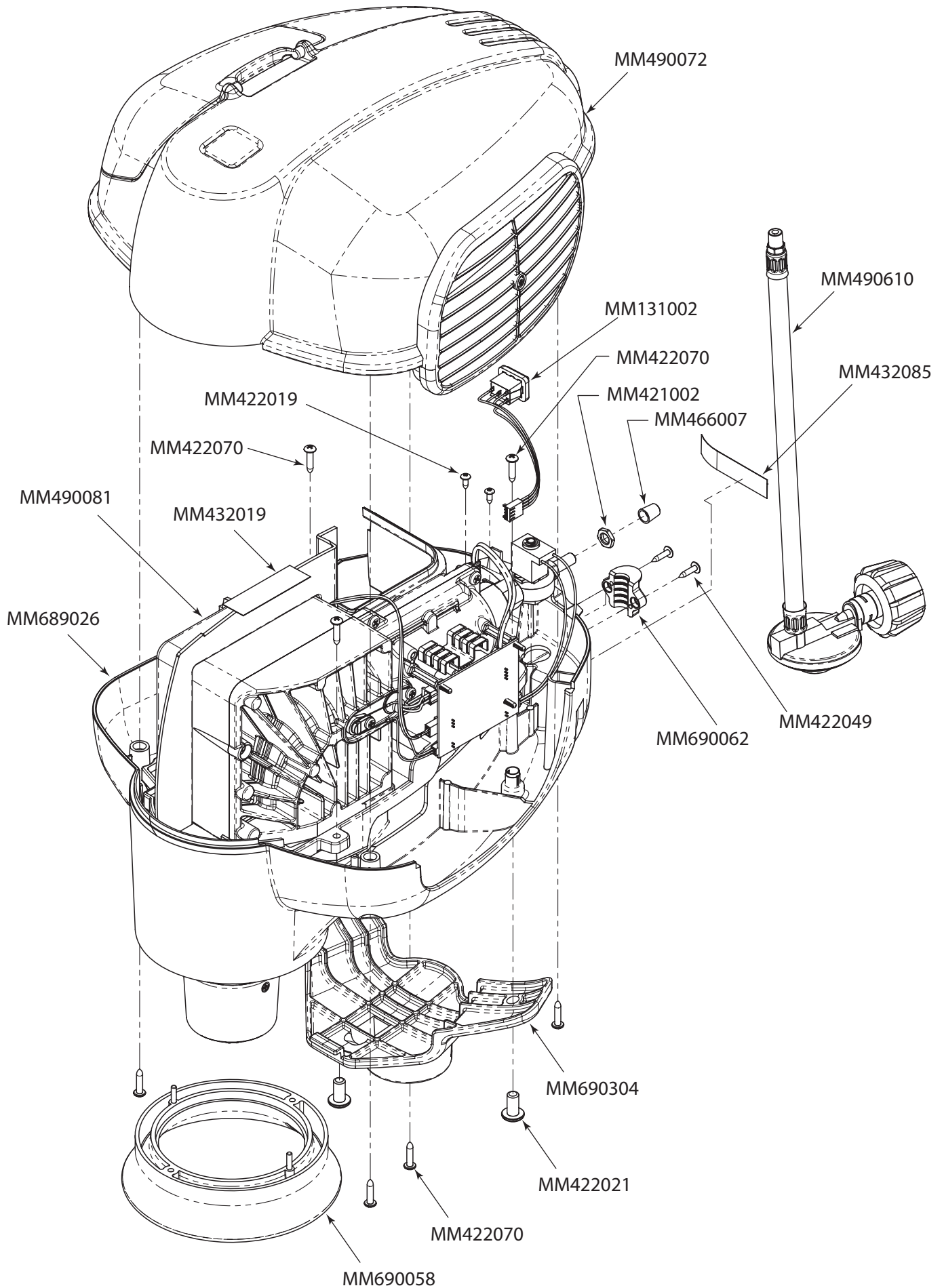
Housing Assy
