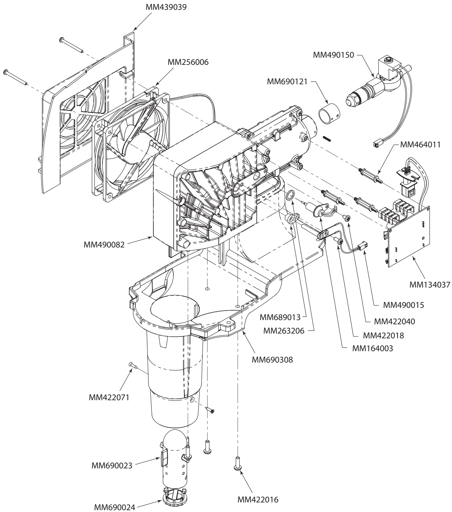
Fan / Heatsink Assy
